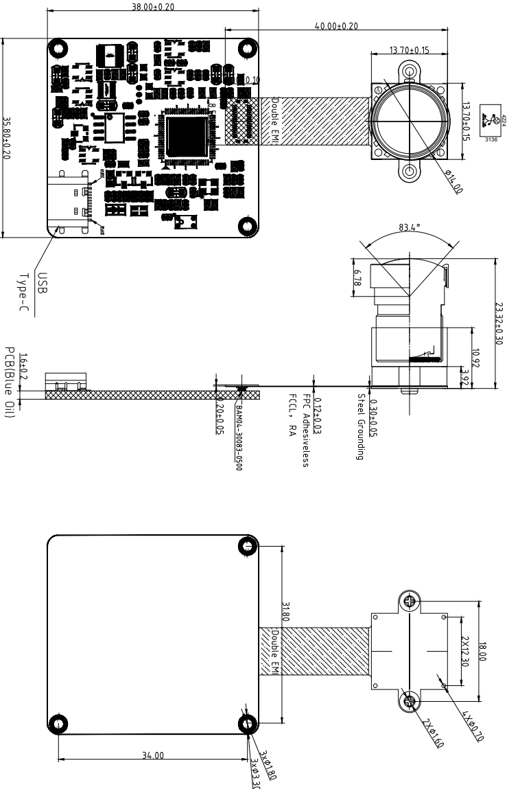
TOP VIEW
